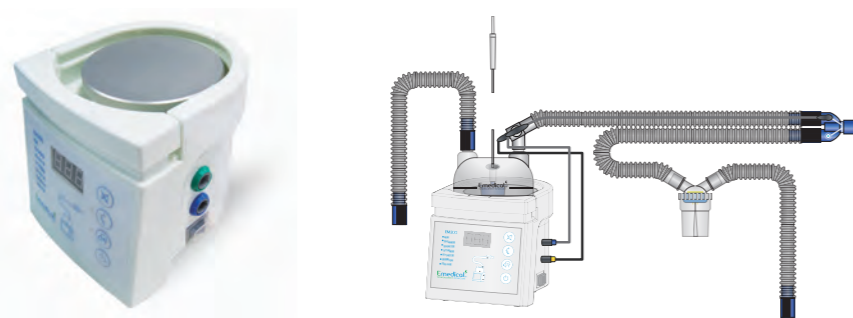
EM200 Automatic Thermostatic Humidifier
